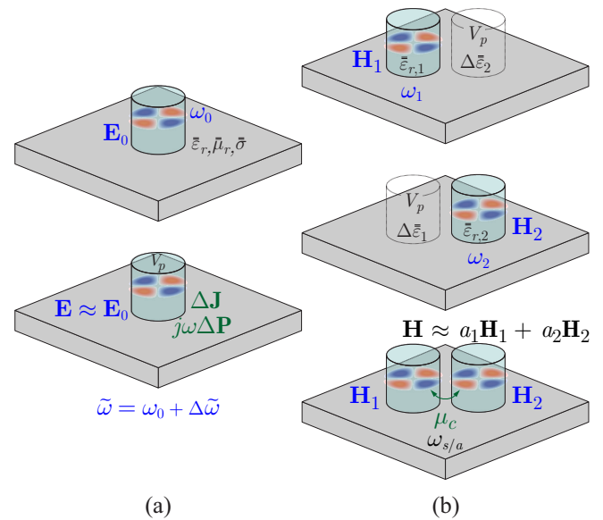
FIG. 15. (a) Material perturbation (induced by the generic quantities j\omega\Delta\mathbf{P} and/or \Delta\mathbf{J} ) and its impact on the resonance frequency of the cavity. (b) Perturbation of a cavity due to coupling with an adjacent one.
